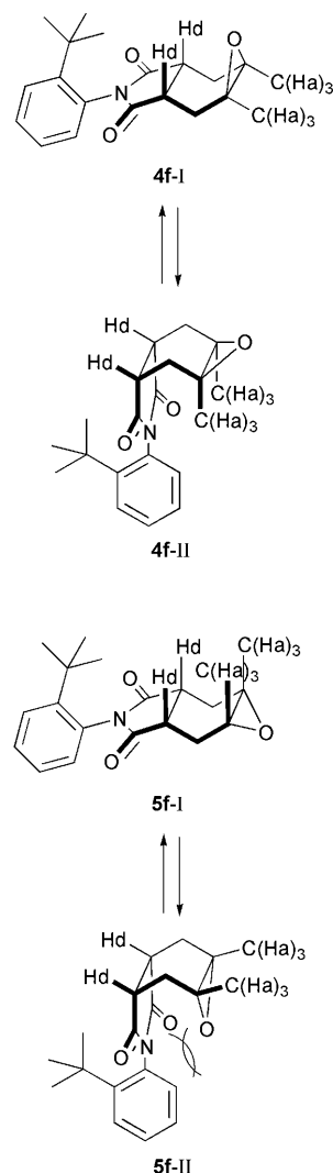
Scheme 2 Flapping of 4f and 5f .
