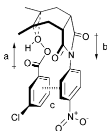
Fig. 3 Interaction between MCPBA and 4-nitrophenyl group of 1e in the transition state. a) Dipole moment of the peracid part [ -C(O)OOH ], b) dipole moment of the imide part ( O=C-N-C=O ), and c) polar/ \pi interaction (||||) between the arenes.
